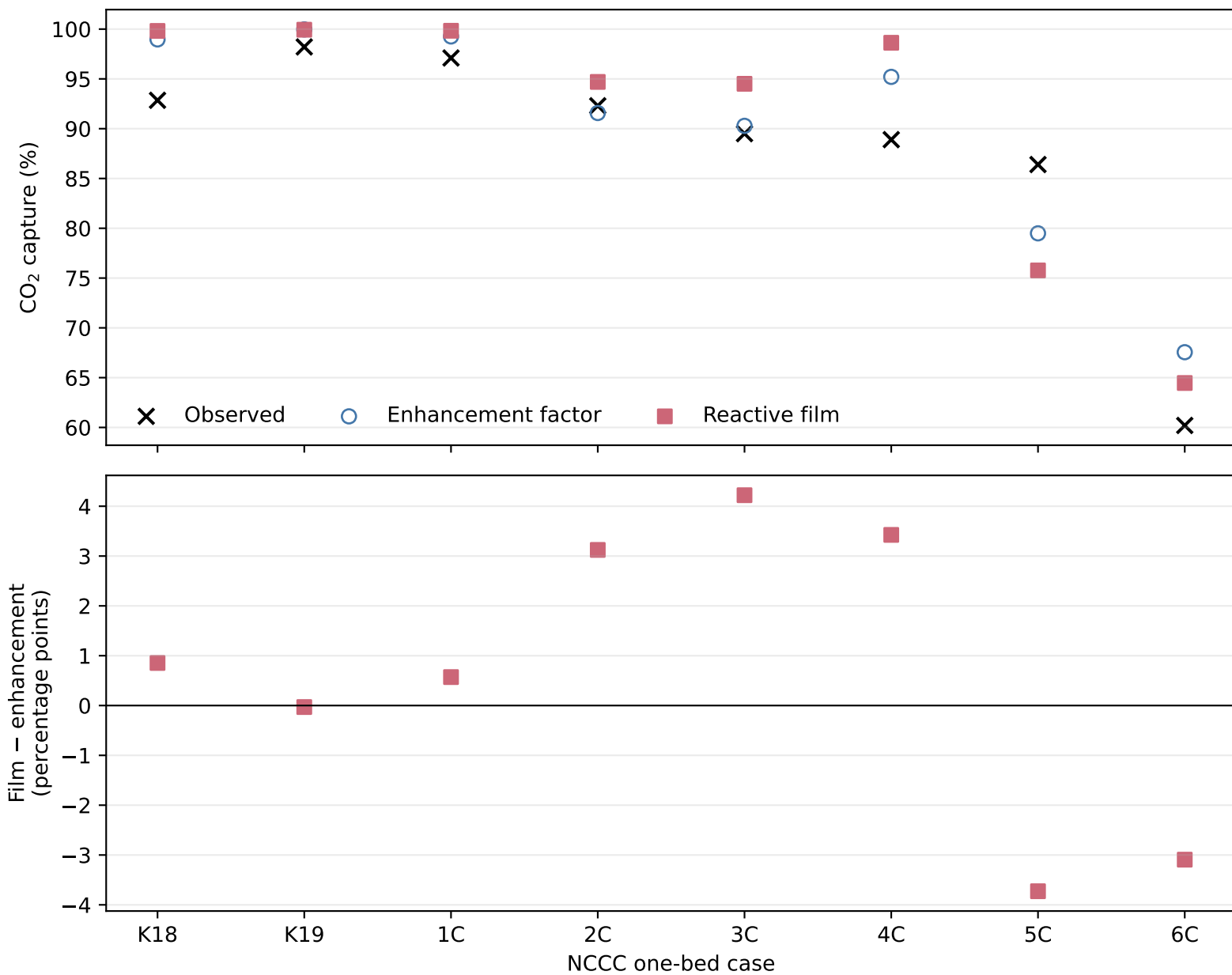
Reactive-film closure changes the predicted capture campaign
