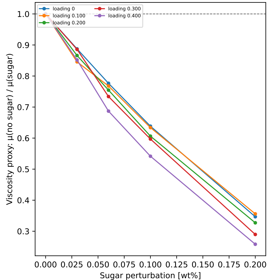
(b) Fixed-chemistry mobility/viscosity perturbation
