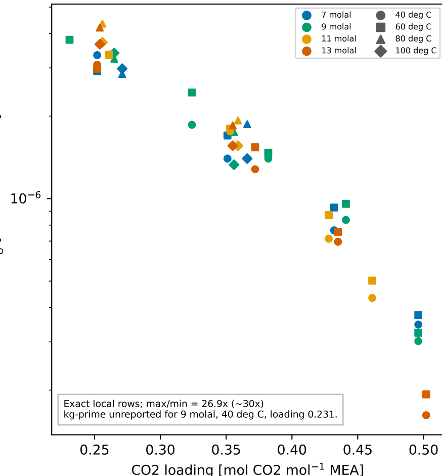
(c) Dugas Table 1 dimensional film evidence
