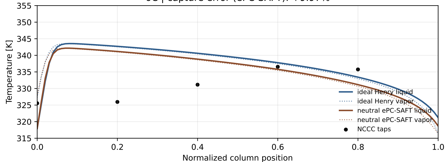
6C | capture error (ePC-SAFT): +9.97%
