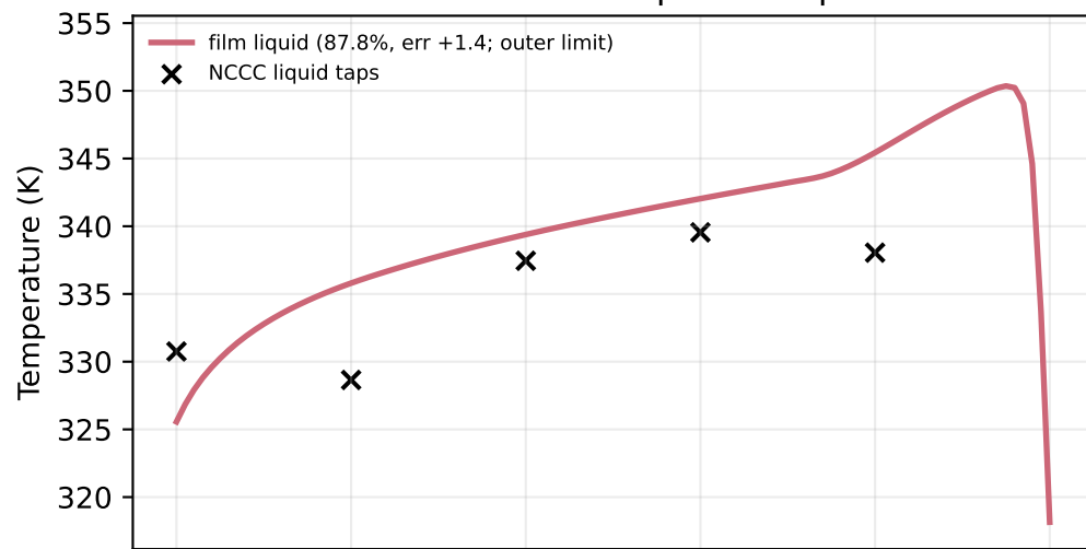
5C reactive-film temperature profile
