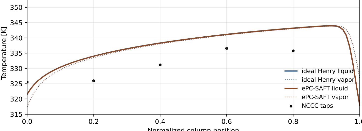
6C | capture error (ePC-SAFT): +9.84%
