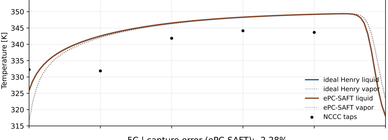
5C | capture error (ePC-SAFT): -2.28%
