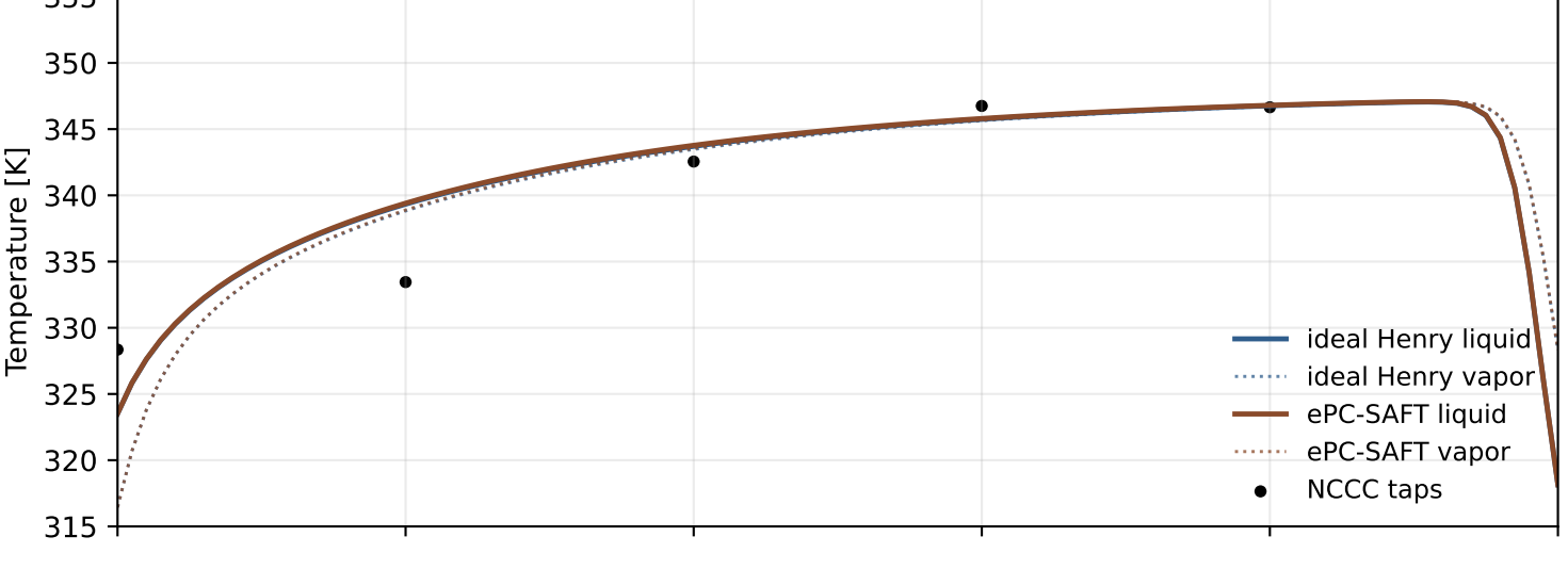
2C | capture error (ePC-SAFT): -6.90%
