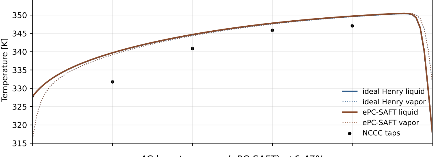
4C | capture error (ePC-SAFT): +6.47%
