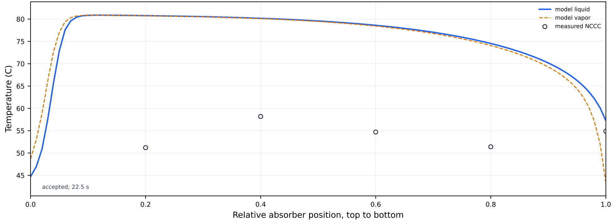
Case 7C: 1 bed, 0 intercoolers
