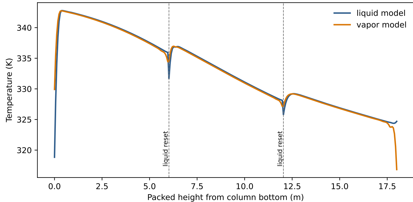
Modeled intercooled temperature profile, NCCC K3
