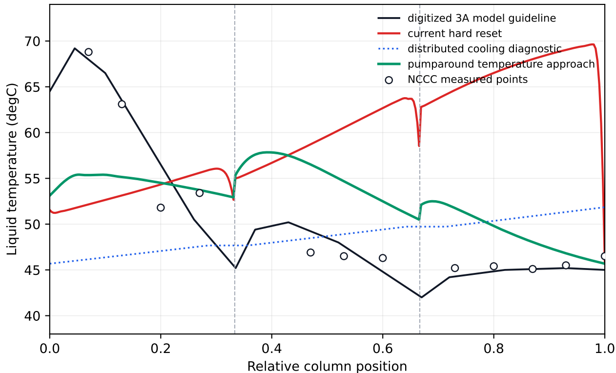
Case 3A/K3 intercooler profile model comparison
