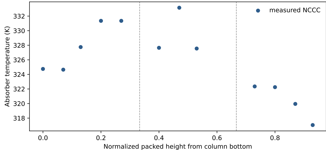
Measured three-bed absorber temperature profile, NCCC 1A
