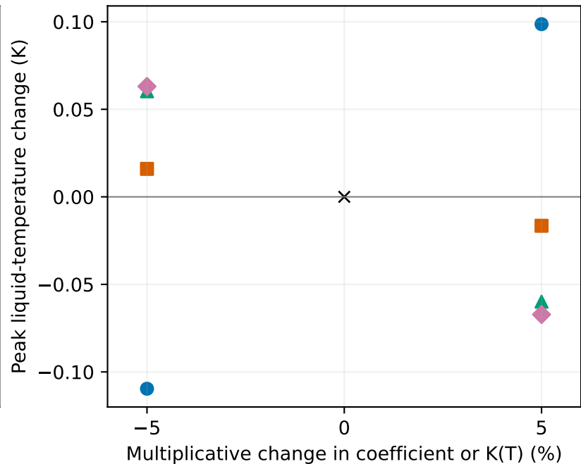
Case 3C: capture and temperature response to thermodynamic inputs
