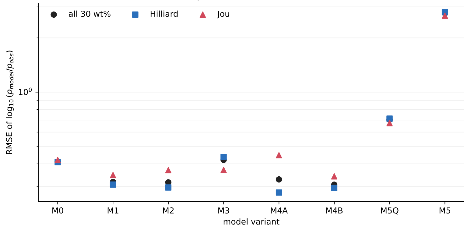
Pressure error by source at 313.15 K and 30 wt% MEA
