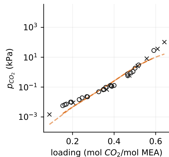
M4A: Hilliard pressure fit RMSE = 0.328
