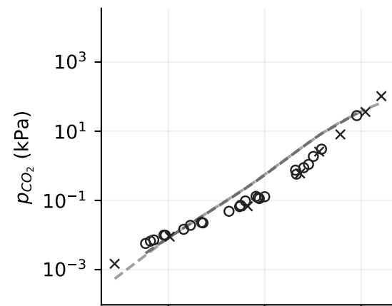
M0: base RMSE = 0.411
