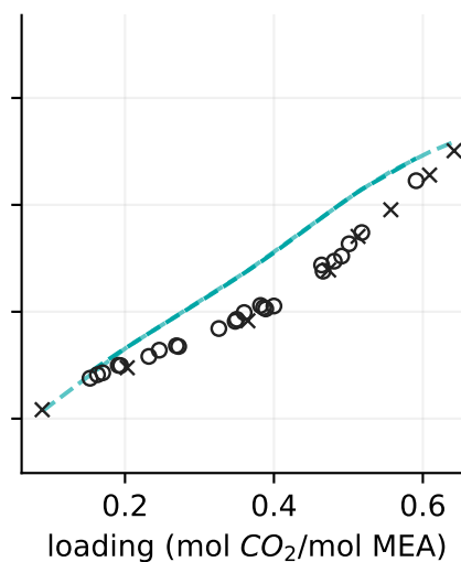
M5Q: M2 + CO 2 QQ RMSE = 0.703
