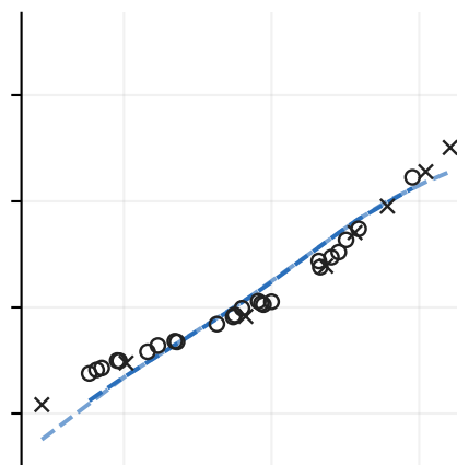
M2: induced association RMSE = 0.316
