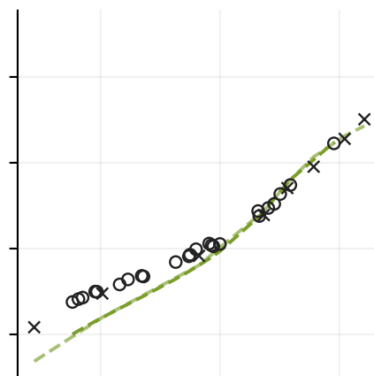
M3: two-row ionic fit RMSE = 0.421
