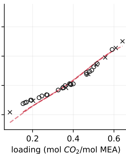
M4B: Hilliard + Jou fit RMSE = 0.306
