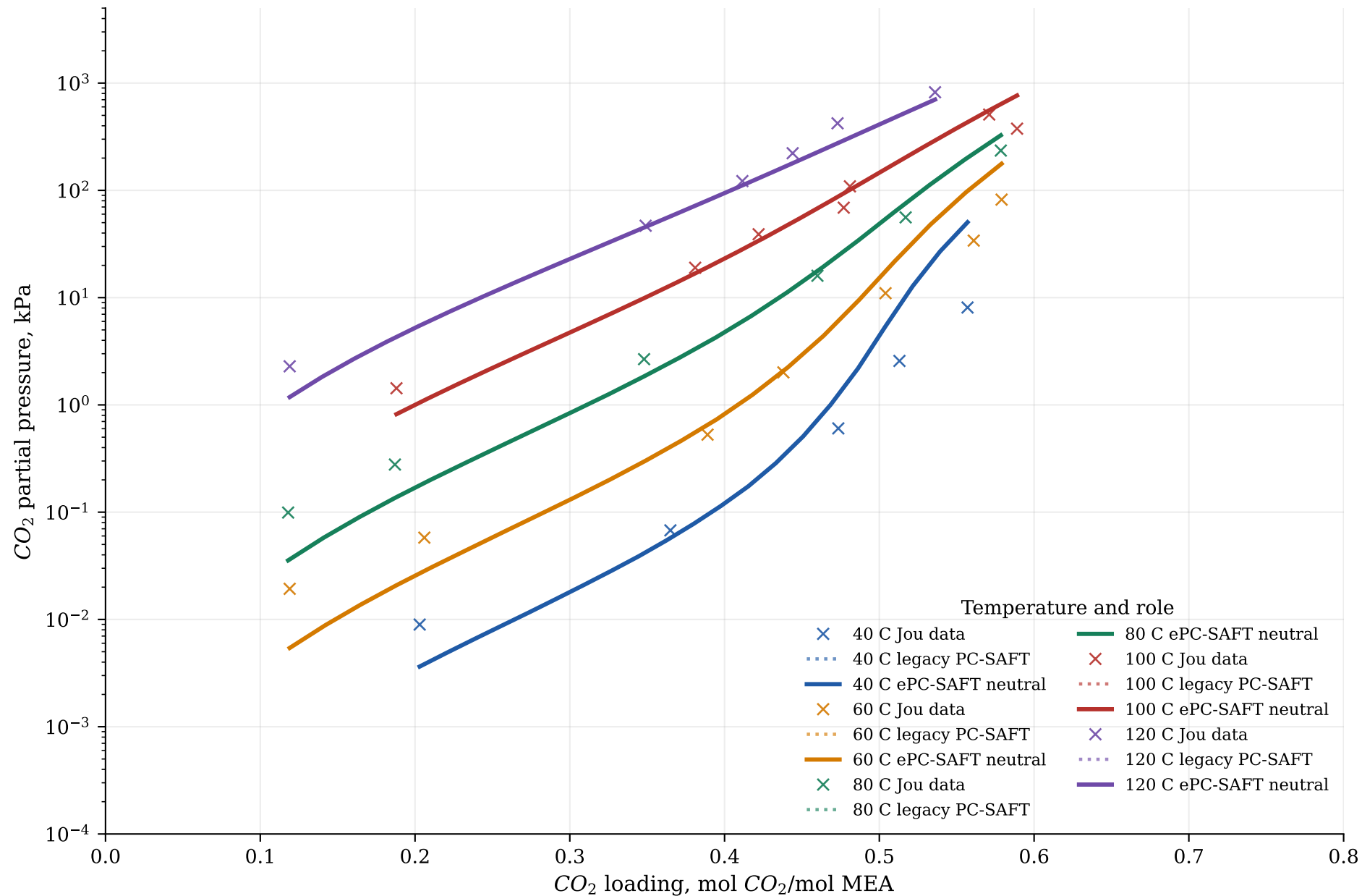
Neutral ePC-SAFT parity against legacy PC-SAFT pressure curves
