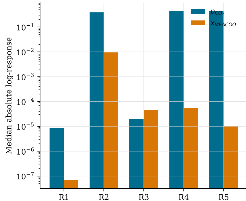
Reaction-constant sensitivities
