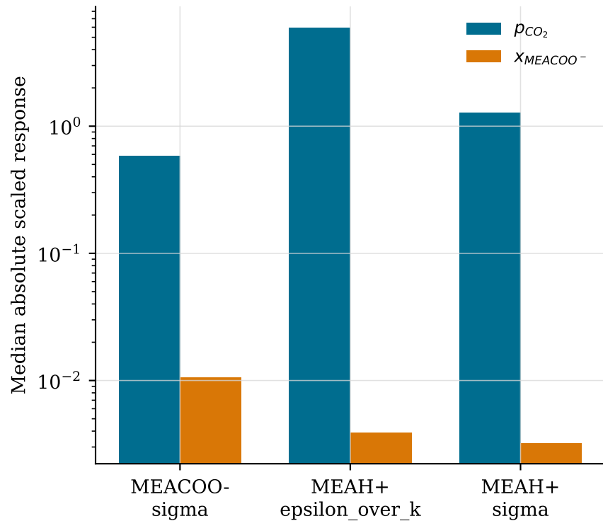
Selected EOS-parameter sensitivities
