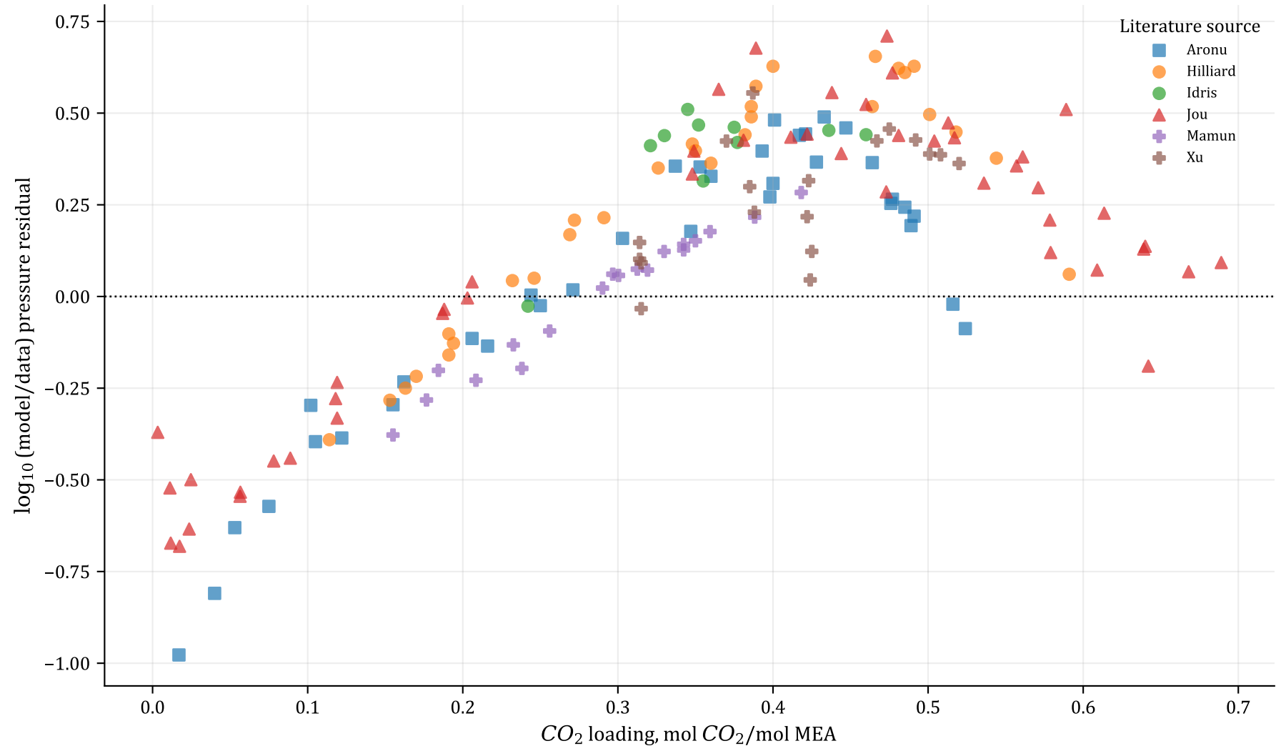
Full-ionic pressure residuals by loading
