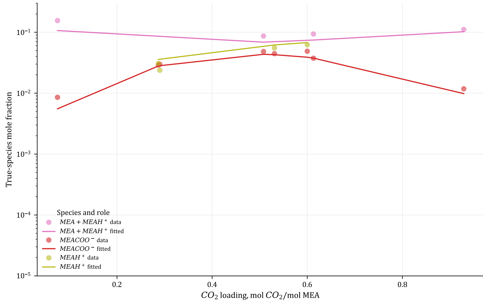
MEA + /MEACOO - loading curves from Tier-A speciation evidence
