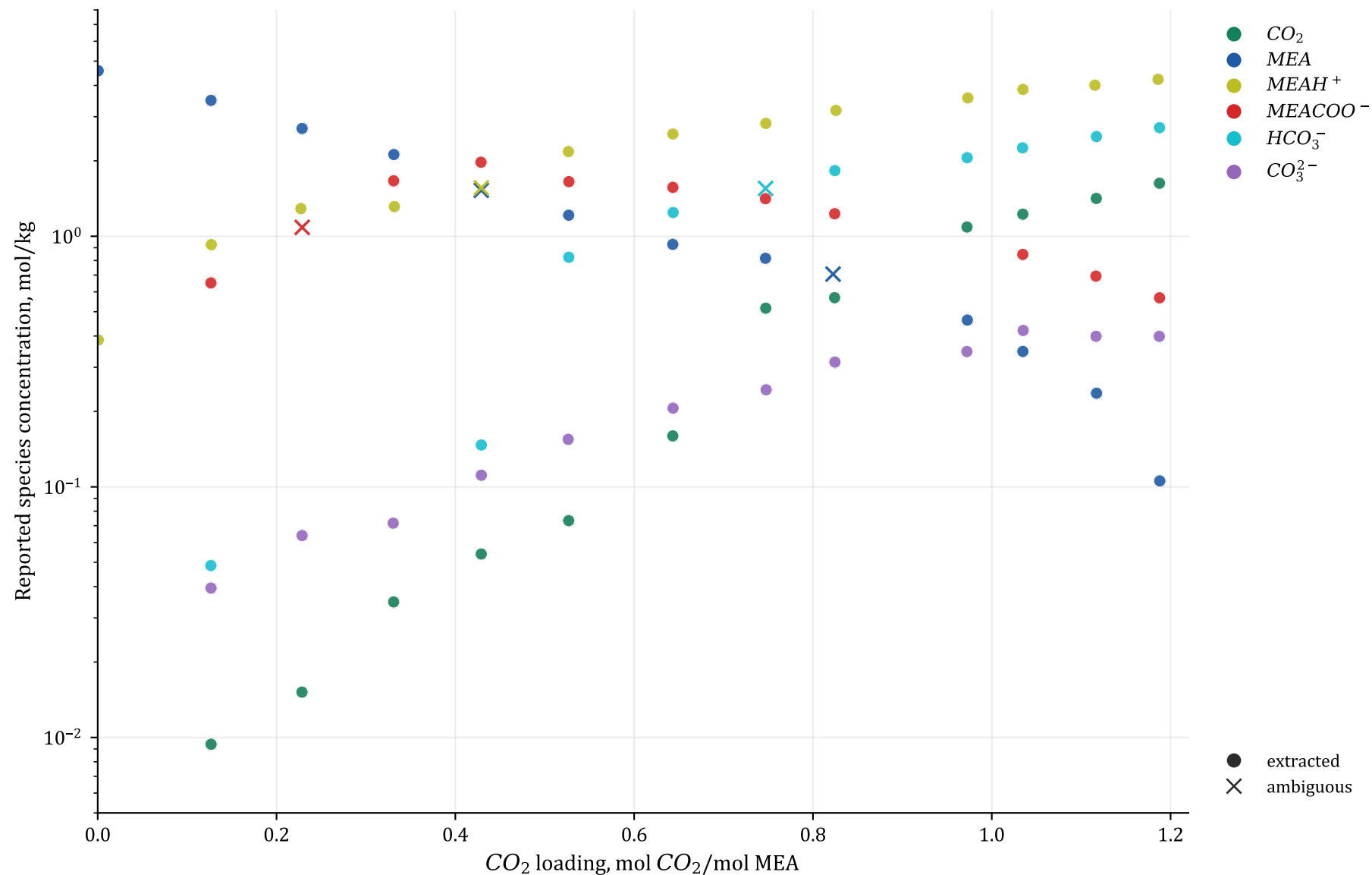
Wong 2015 Raman speciation, 30 wt% MEA at 30 °C
