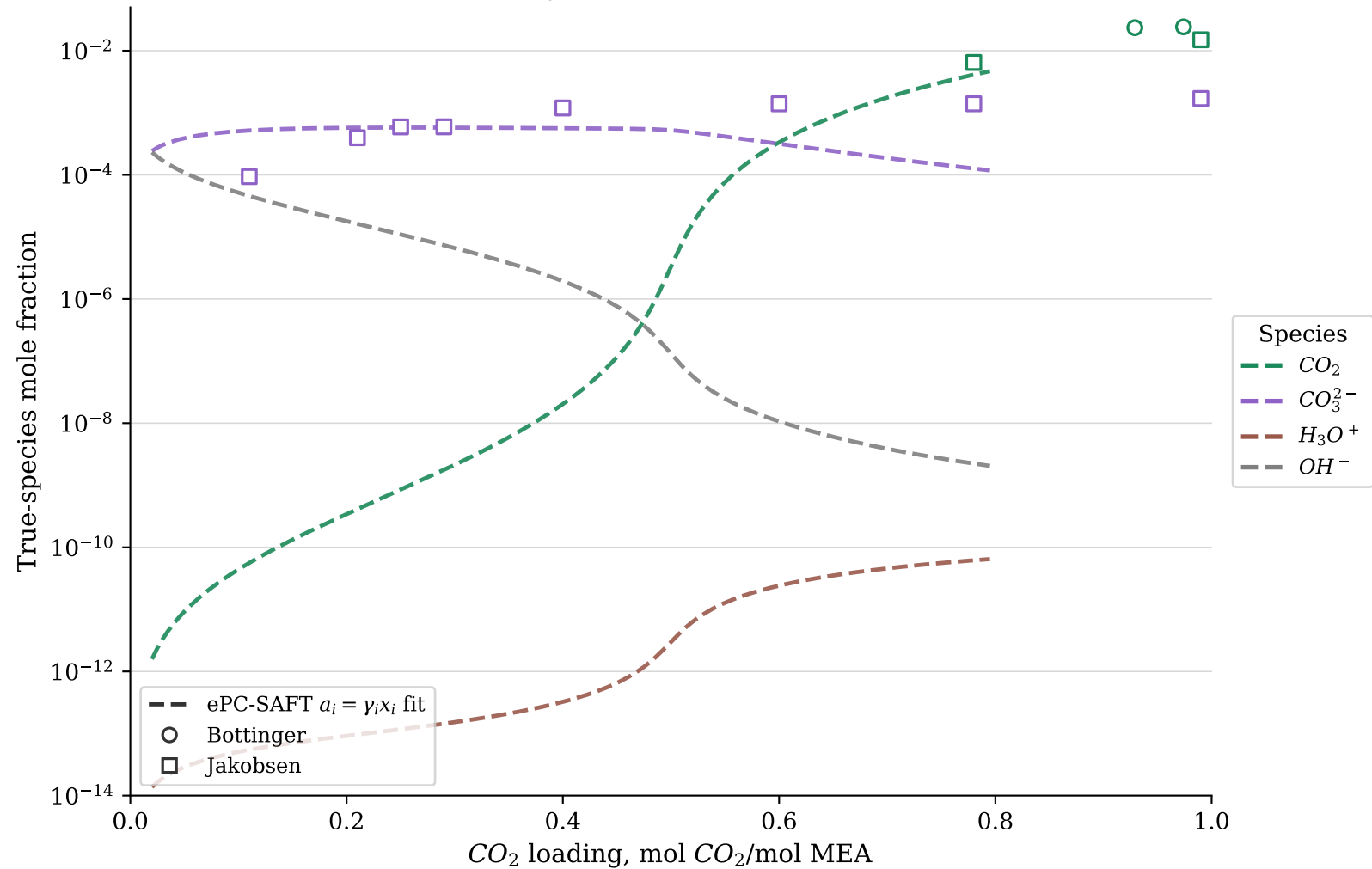
Nonideal ePC-SAFT activity speciation, trace and minor species, 20 C
