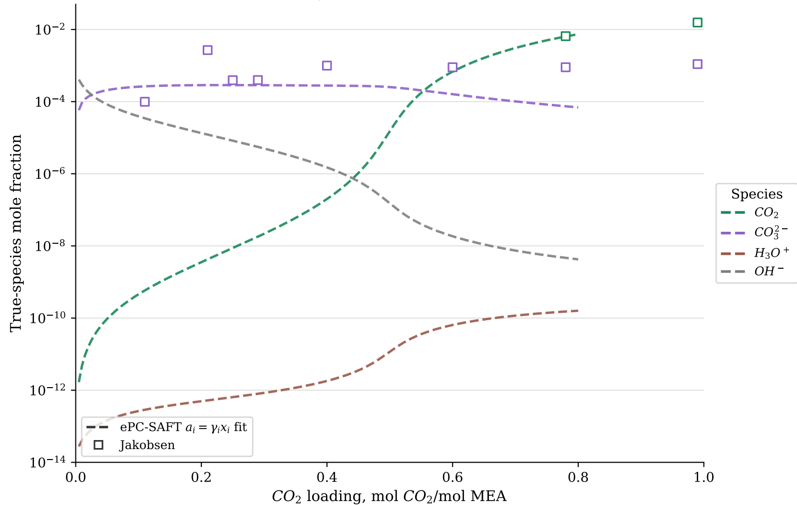
Nonideal ePC-SAFT activity speciation, trace and minor species, 40 C
