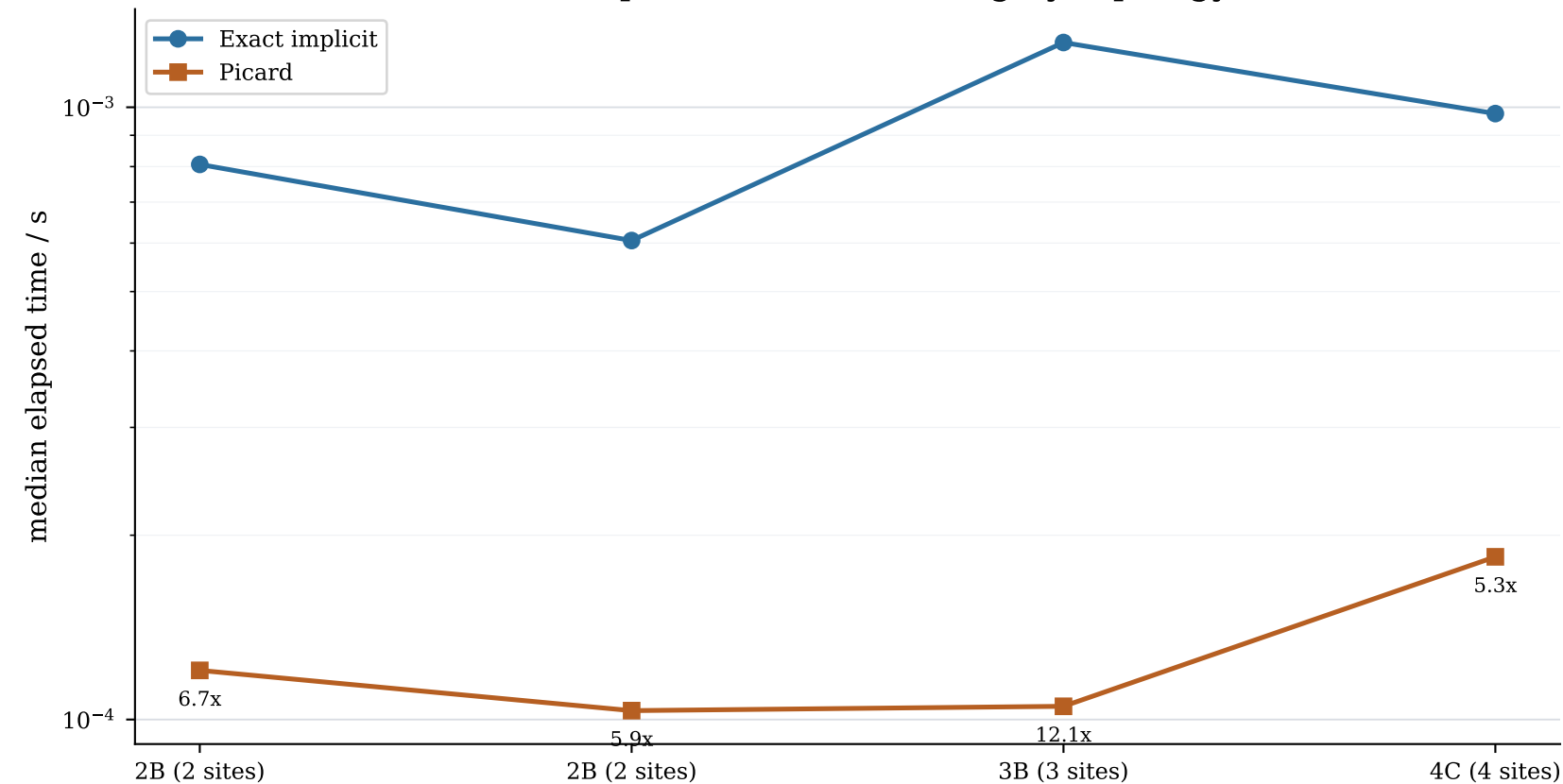
Exact implicit vs Picard timing by topology
