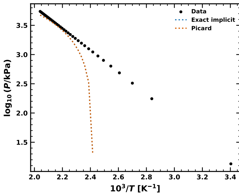
Methanol
