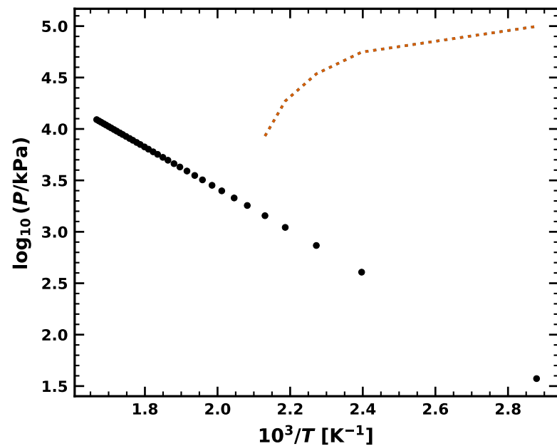
Water
