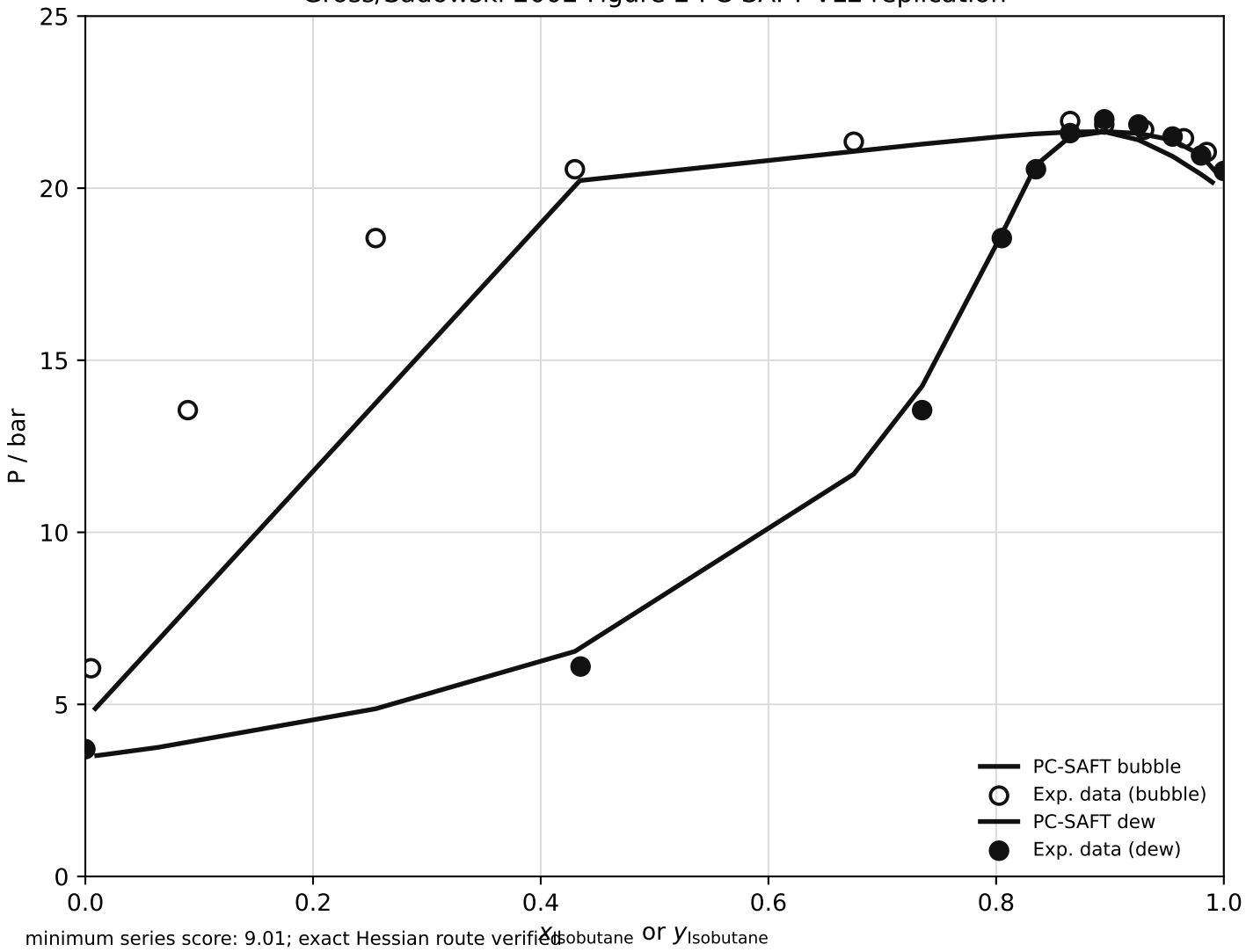
Gross/Sadowski 2002 Figure 2 PC-SAFT VLE replication
