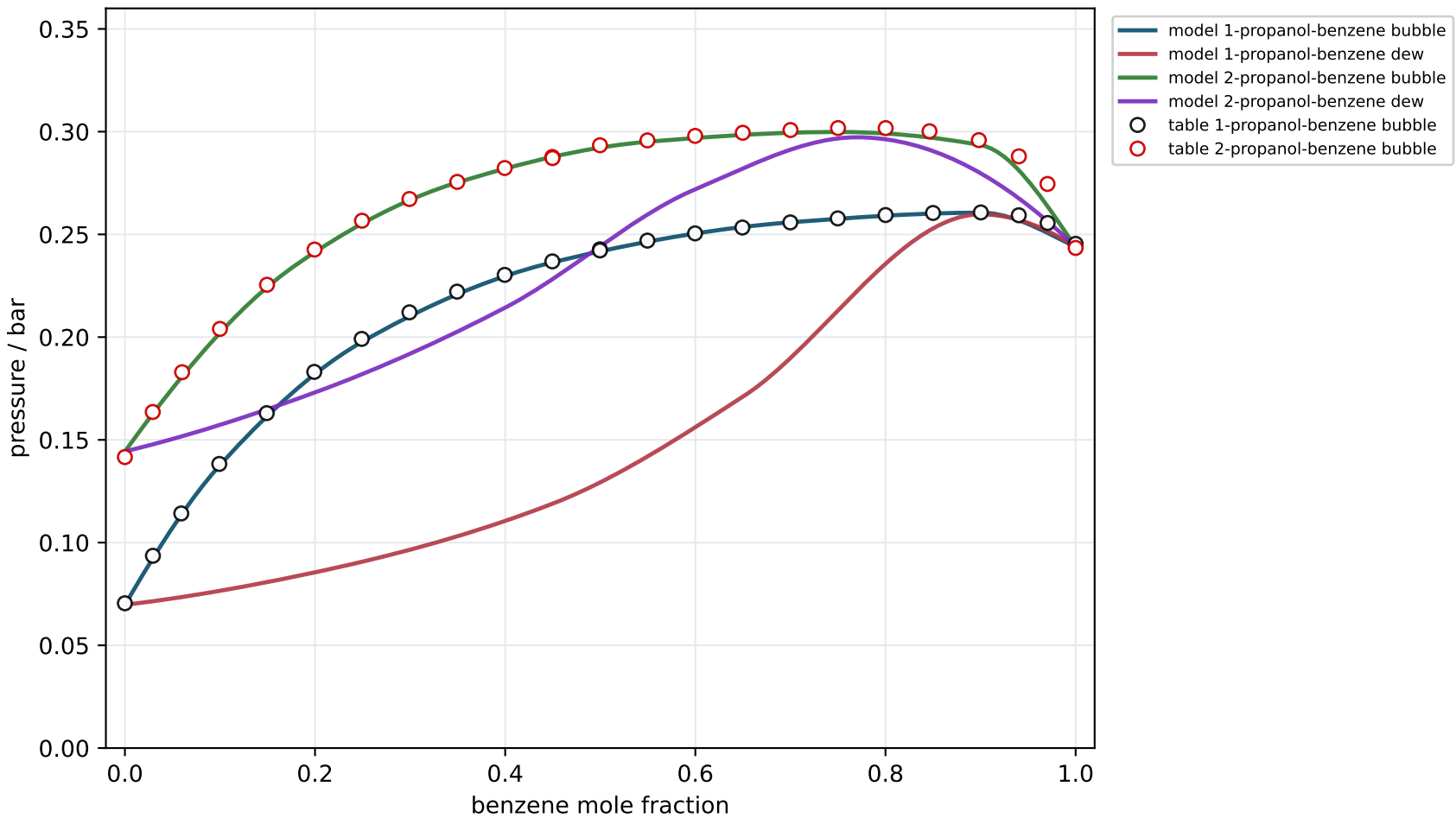
Gross 2002 Fig. 5: propanol/benzene at 40 C
