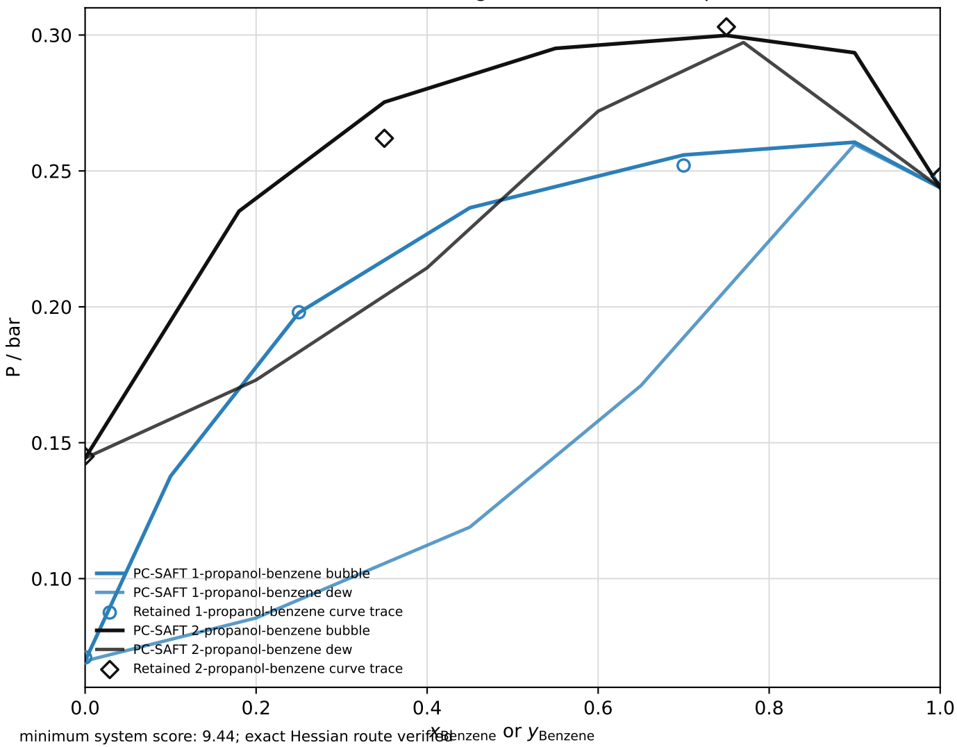
Gross/Sadowski 2002 Figure 5 PC-SAFT VLE replication
