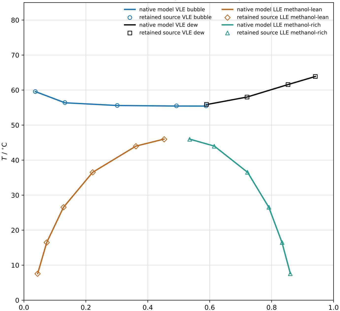
Gross/Sadowski 2002 Figure 8 PC-SAFT replication
