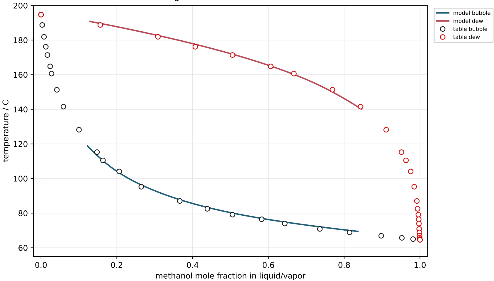
Gross 2002 Fig. 9: methanol/1-octanol at 1.013 bar
