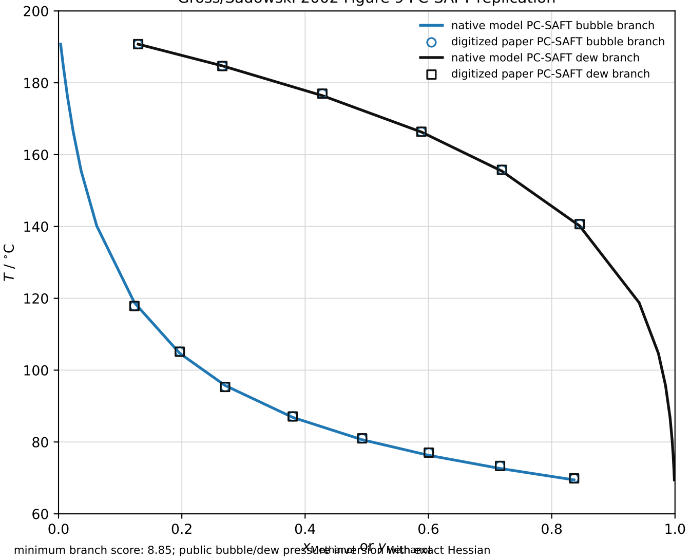
Gross/Sadowski 2002 Figure 9 PC-SAFT replication
