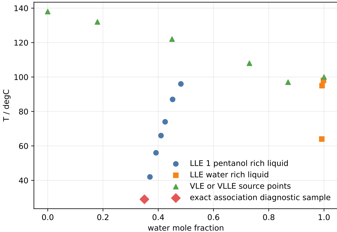
Gross 2002 Figure 10 cross-association stress mirror
