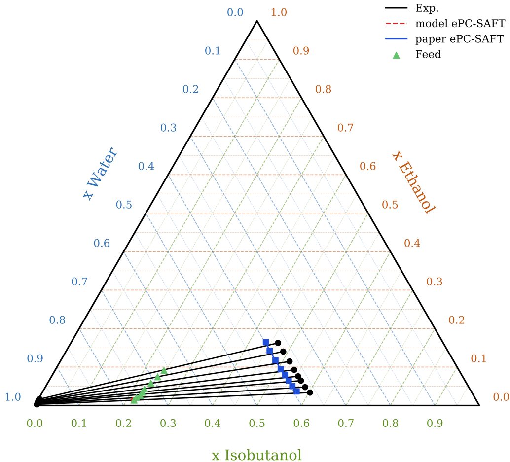
Figure 2. LLE for the system water + ethanol + isobutanol + 5 wt % NaCl at 293.15 K and atmospheric pressure expressed as salt-free composition: black (exp), red dashed (package public ePC-SAFT, 1/8 tie-lines), blue squares (paper ePC-SAFT organic branch, 8 points), and green (feed compositions).
