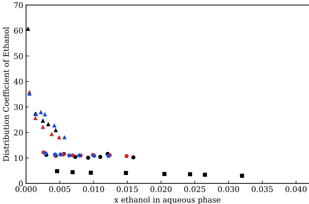
Figure 9. Distribution coefficient of ethanol over water of the mixture water + ethanol + isobutanol + NaCl; black (293.15 K), red (303.15 K), blue (313.15 K), squares (without NaCl), circles (5 wt % NaCl), and triangles (10 wt % NaCl).
