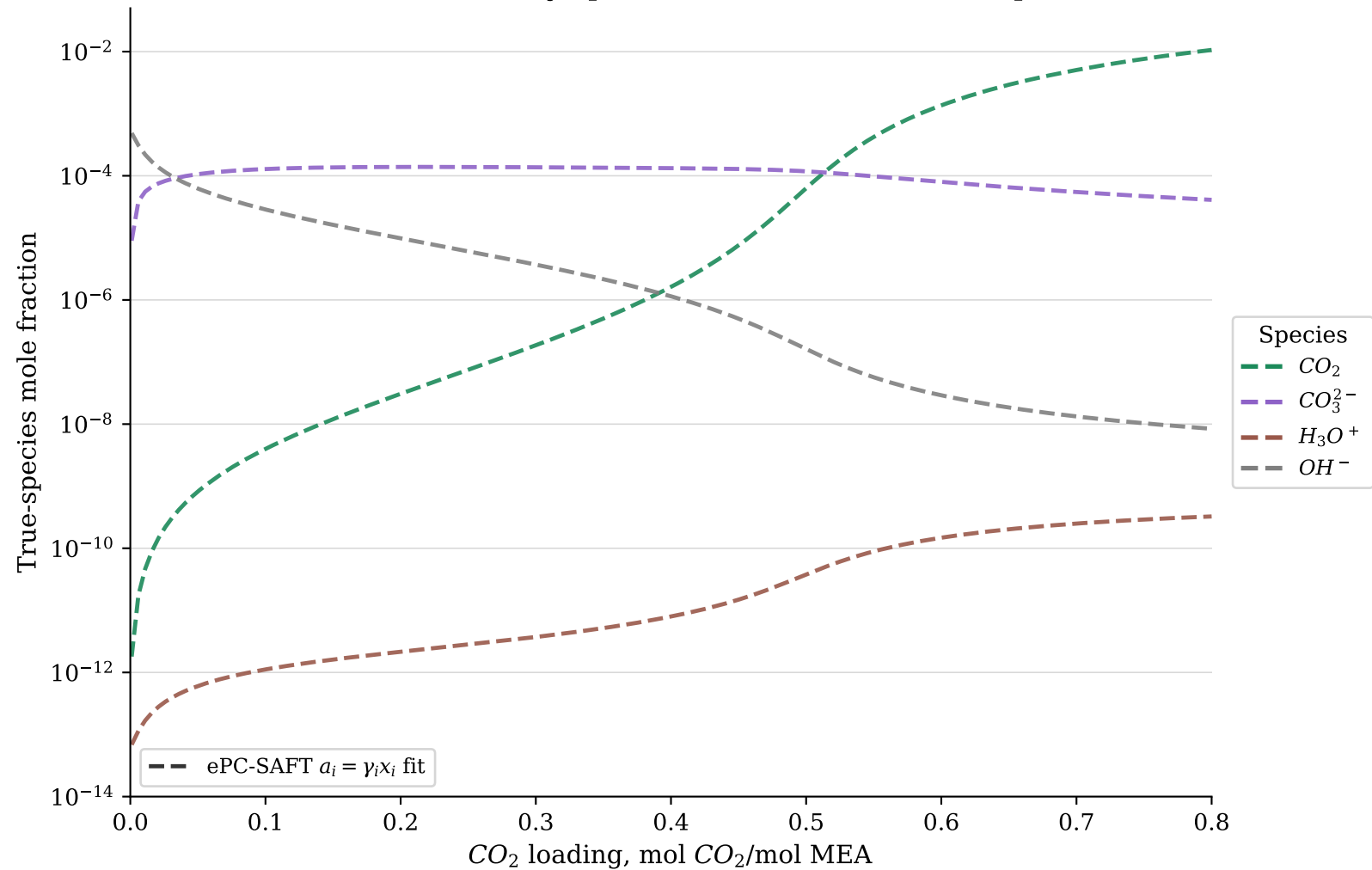
Nonideal ePC-SAFT activity speciation, trace and minor species, 60 C
