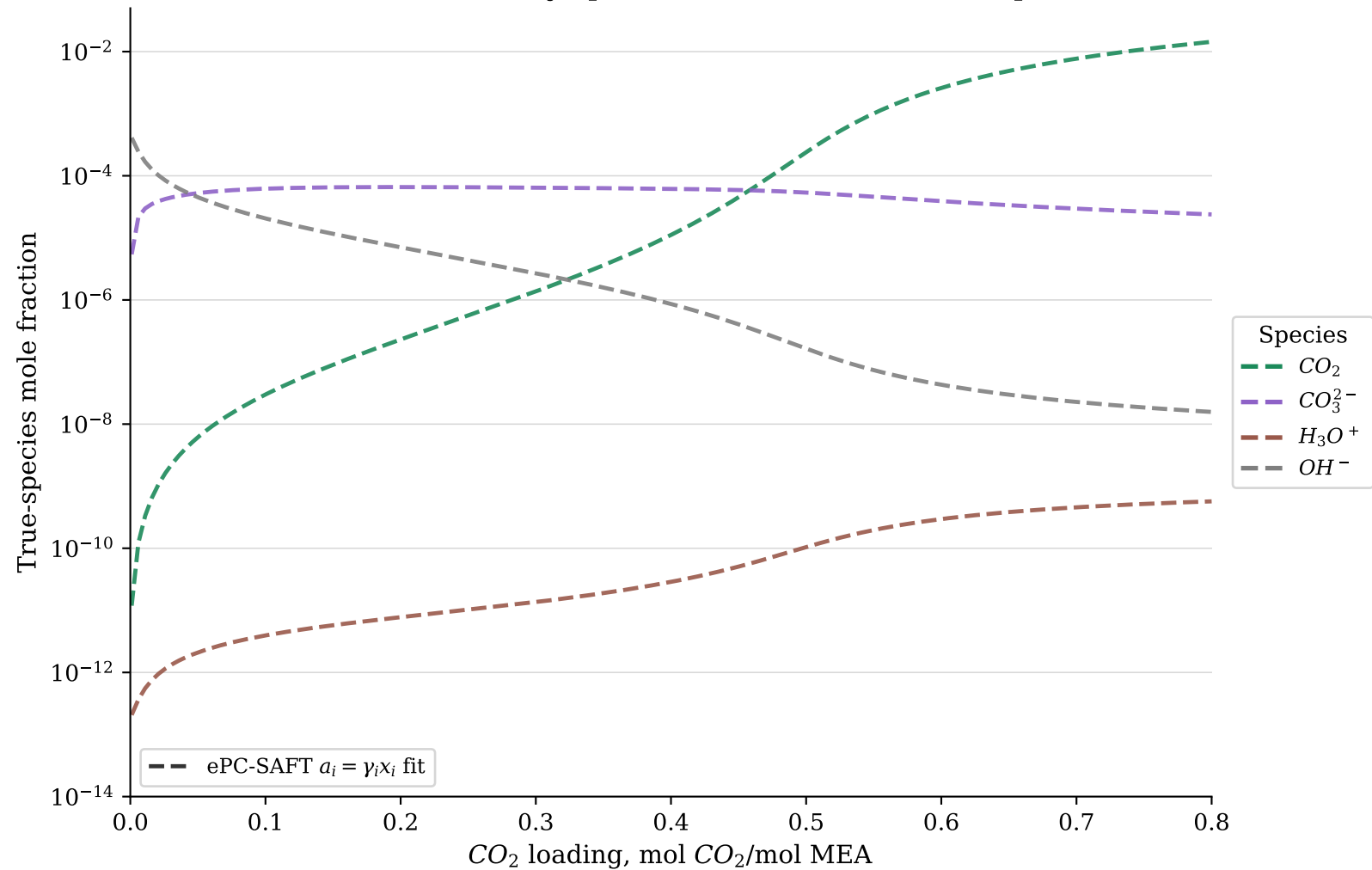
Nonideal ePC-SAFT activity speciation, trace and minor species, 80 C
