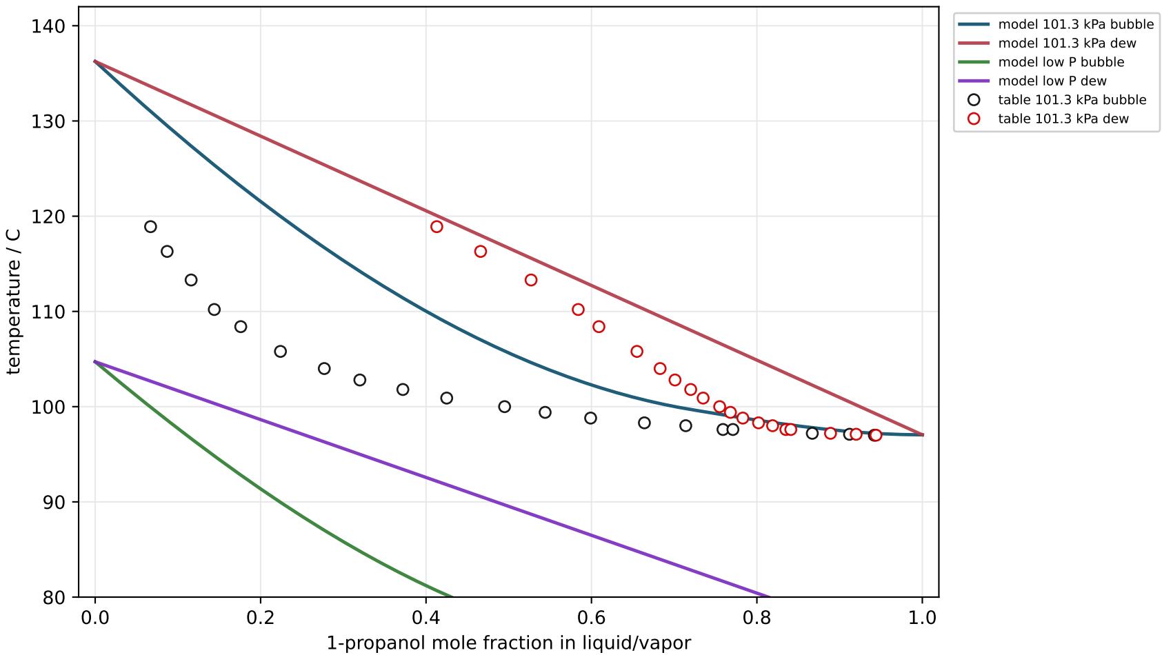
Gross 2002 Fig. 3: 1-propanol/ethylbenzene
