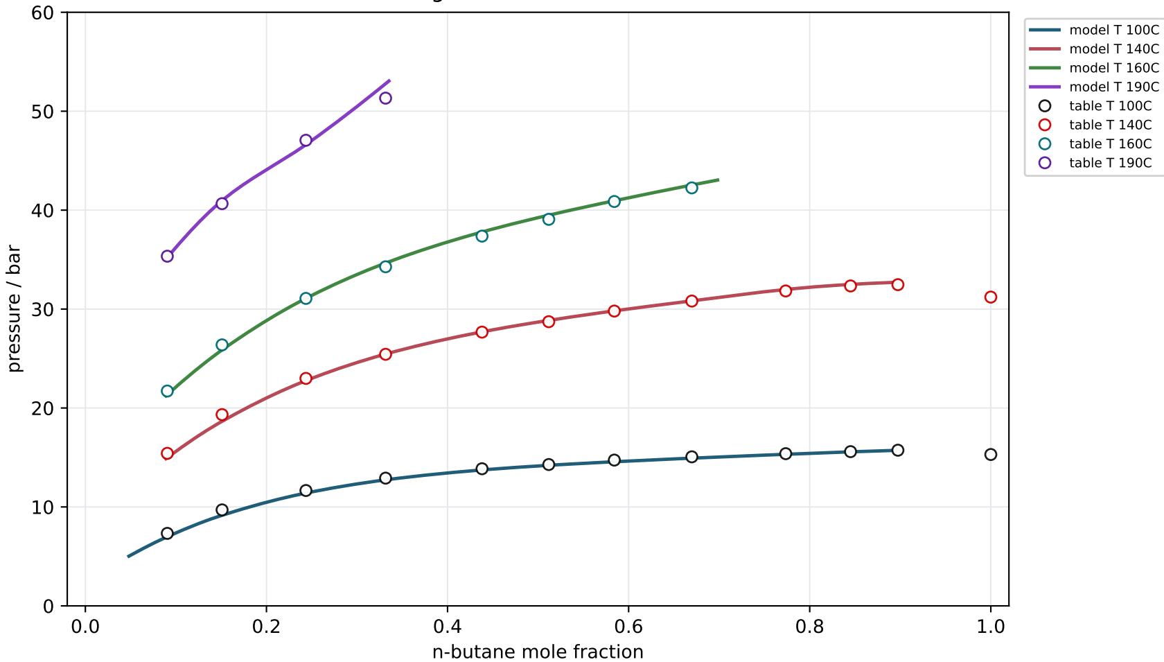
Gross 2002 Fig. 7: ethanol/n-butane isotherms
