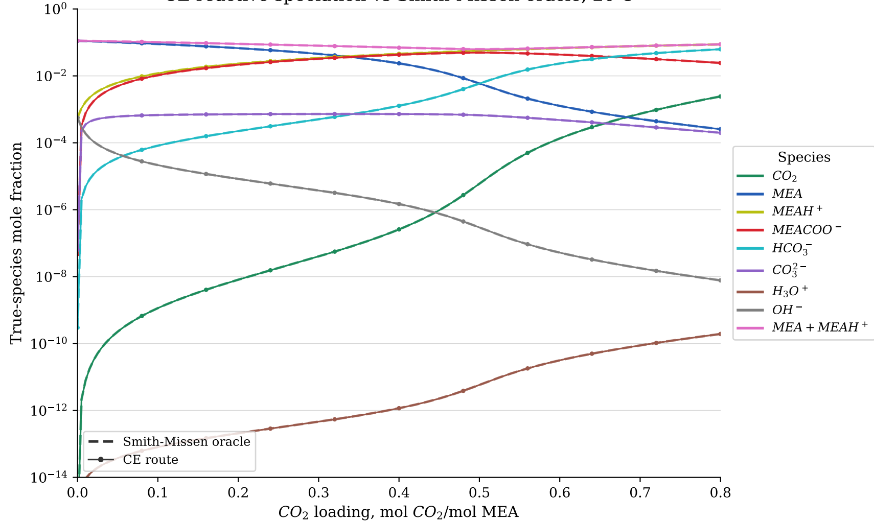
CE reactive speciation vs Smith-Missen oracle, 20 C
