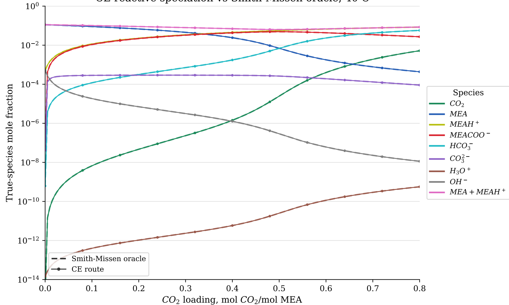
CE reactive speciation vs Smith-Missen oracle, 40 C
