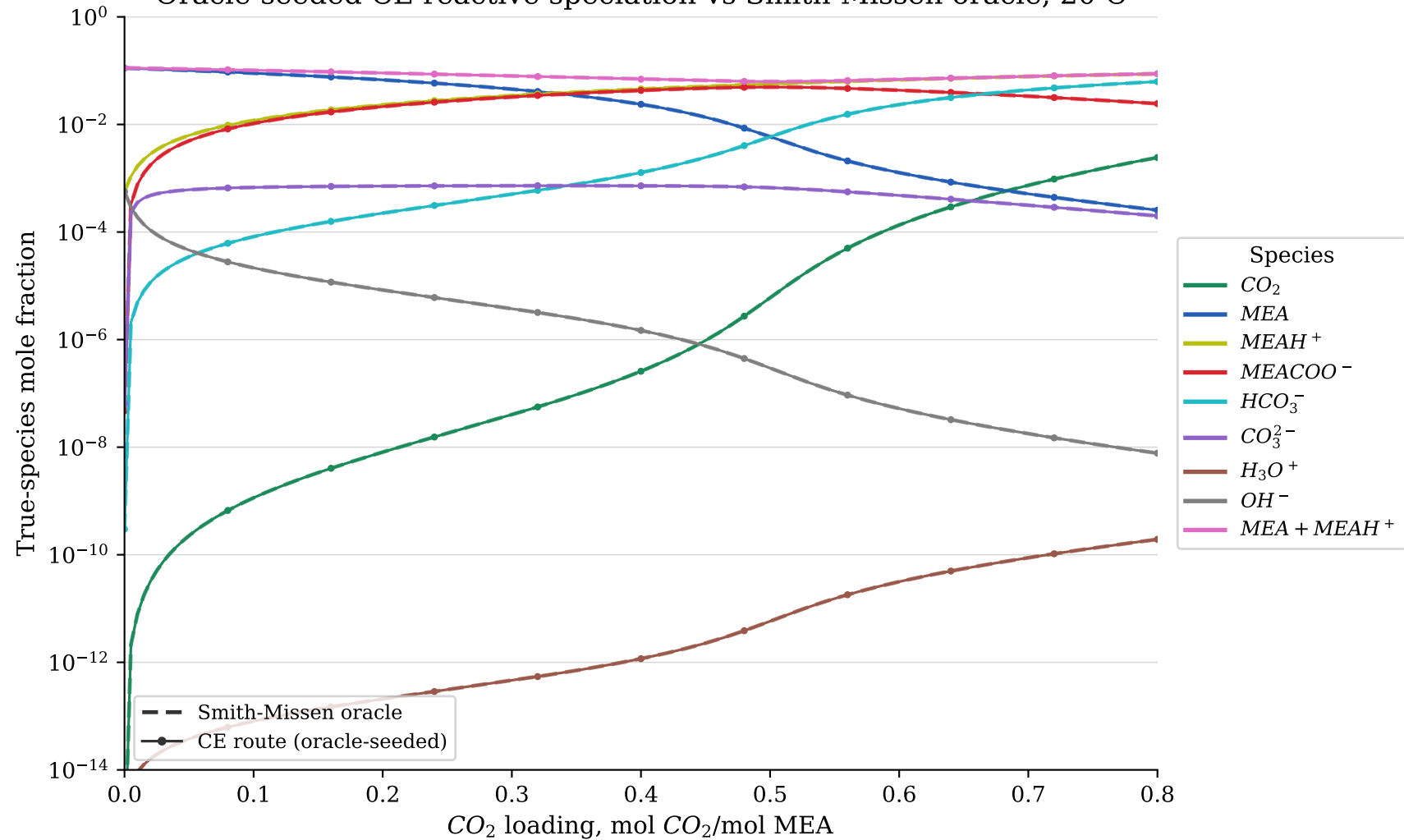
Oracle-seeded CE reactive speciation vs Smith-Missen oracle, 20 C
