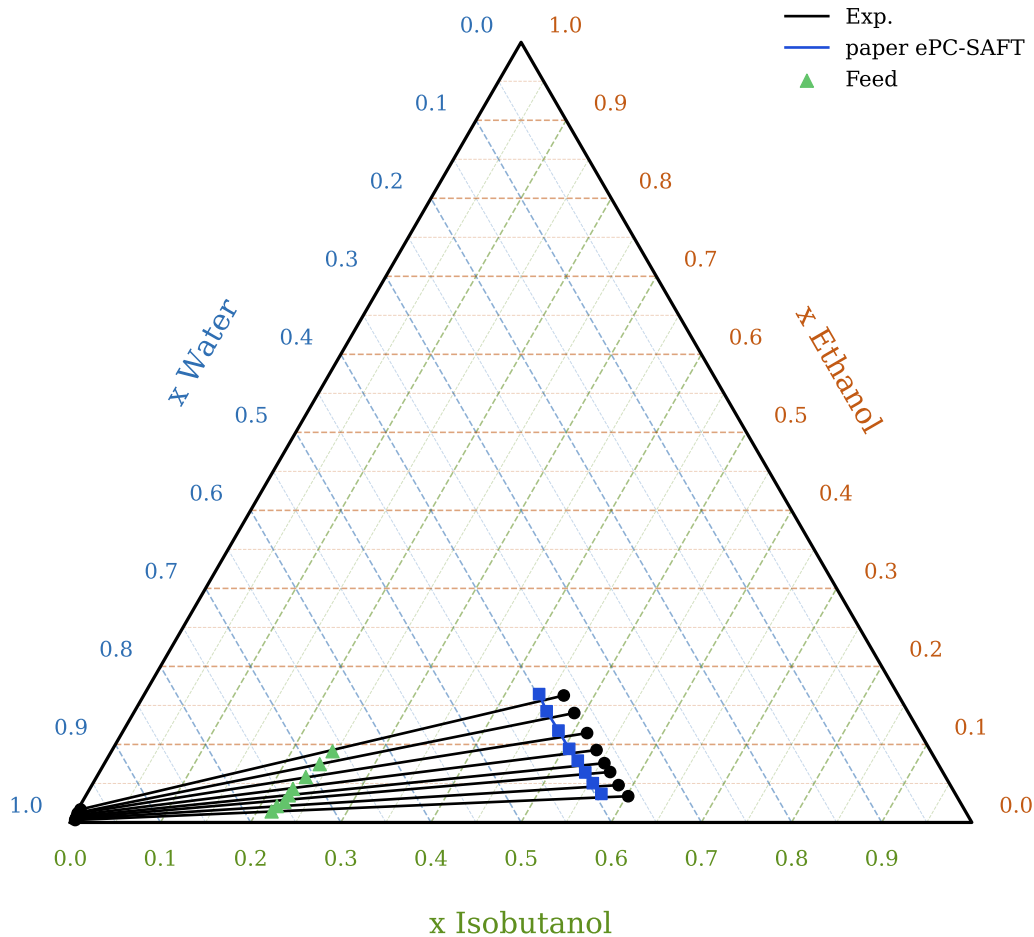
Figure 2. LLE for the system water + ethanol + isobutanol + 5 wt % NaCl at 293.15 K and atmospheric pressure expressed as salt-free composition: black (exp), package public ePC-SAFT rejected all model tie-lines; no red model tie-lines are drawn, blue squares (paper ePC-SAFT organic branch, 8 points), and green (feed compositions).
