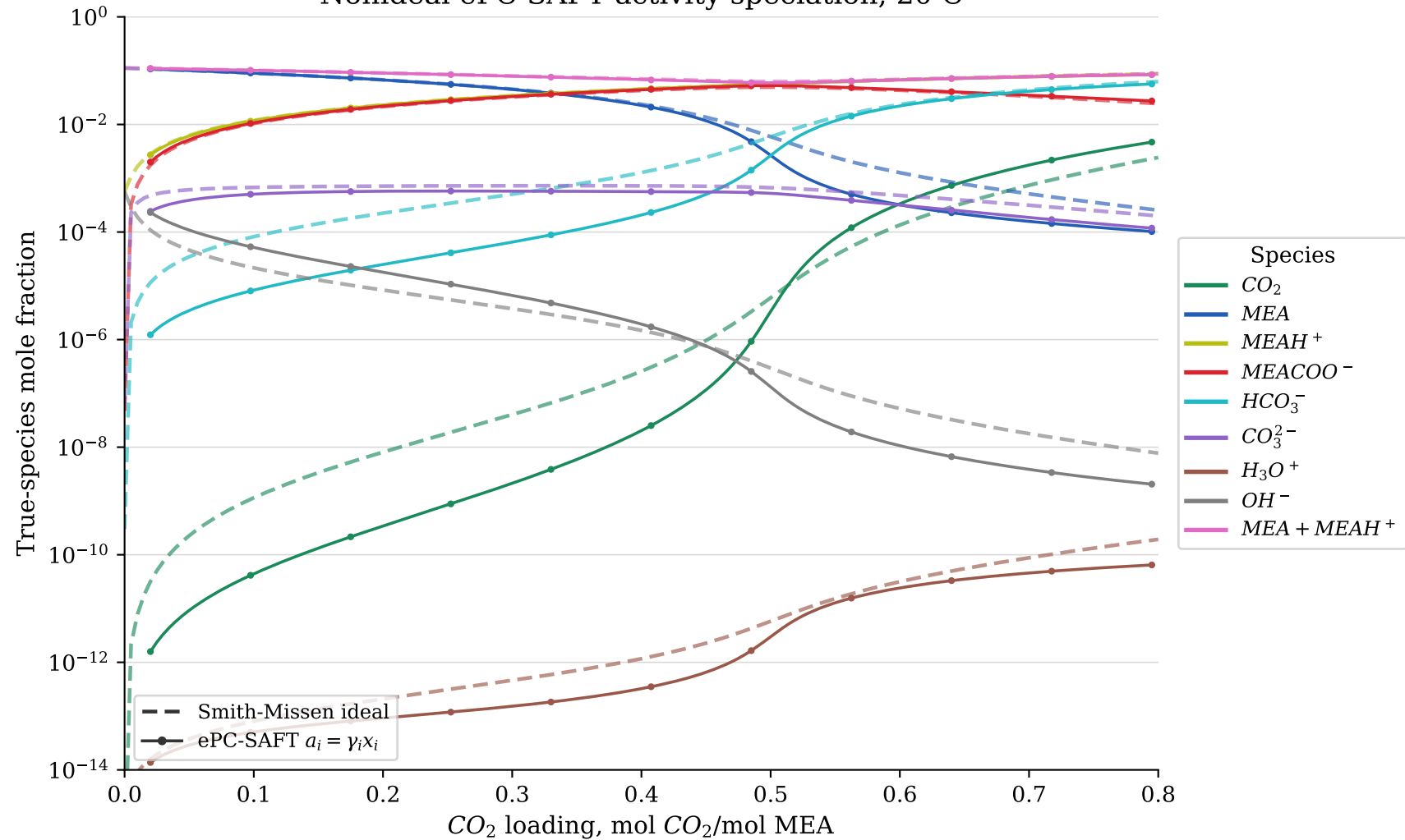
Nonideal ePC-SAFT activity speciation, 20 C
