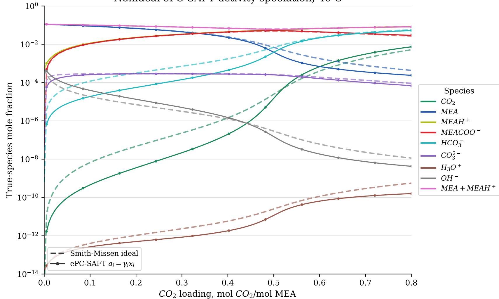
Nonideal ePC-SAFT activity speciation, 40 C
