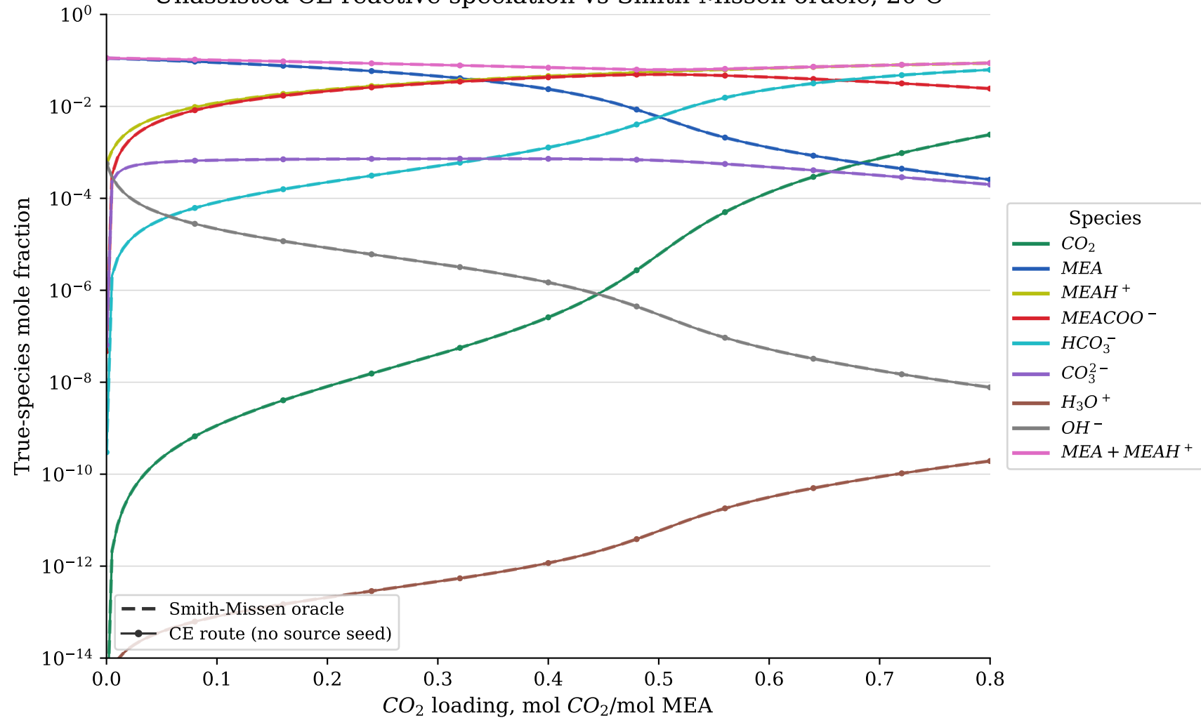
Unassisted CE reactive speciation vs Smith-Missen oracle, 20 C
