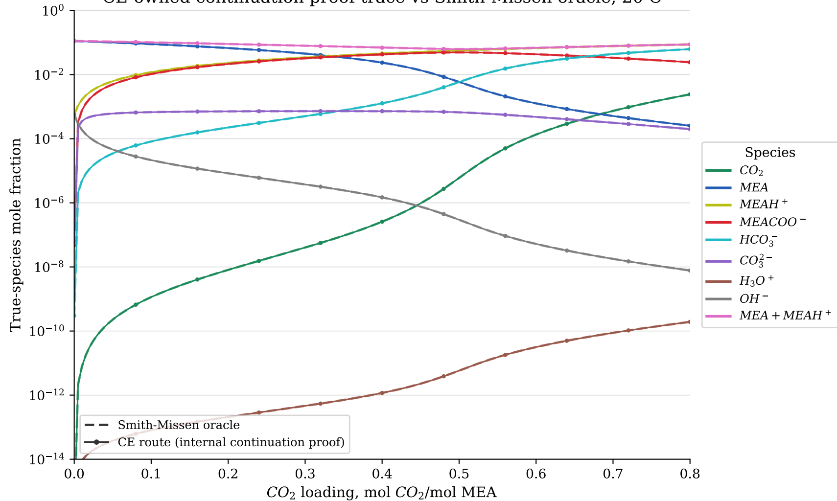
CE-owned continuation proof trace vs Smith-Missen oracle, 20 C
