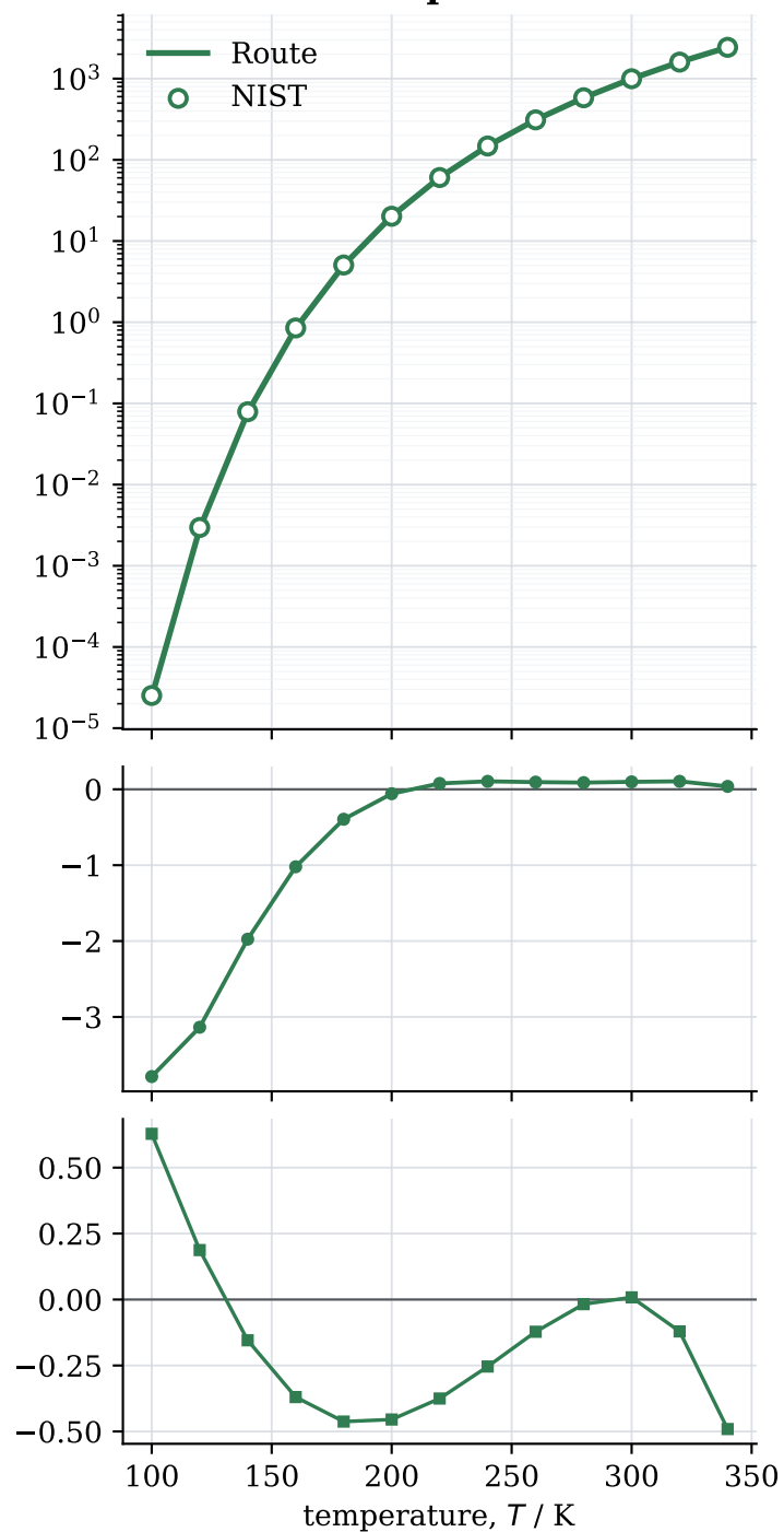
Propane
