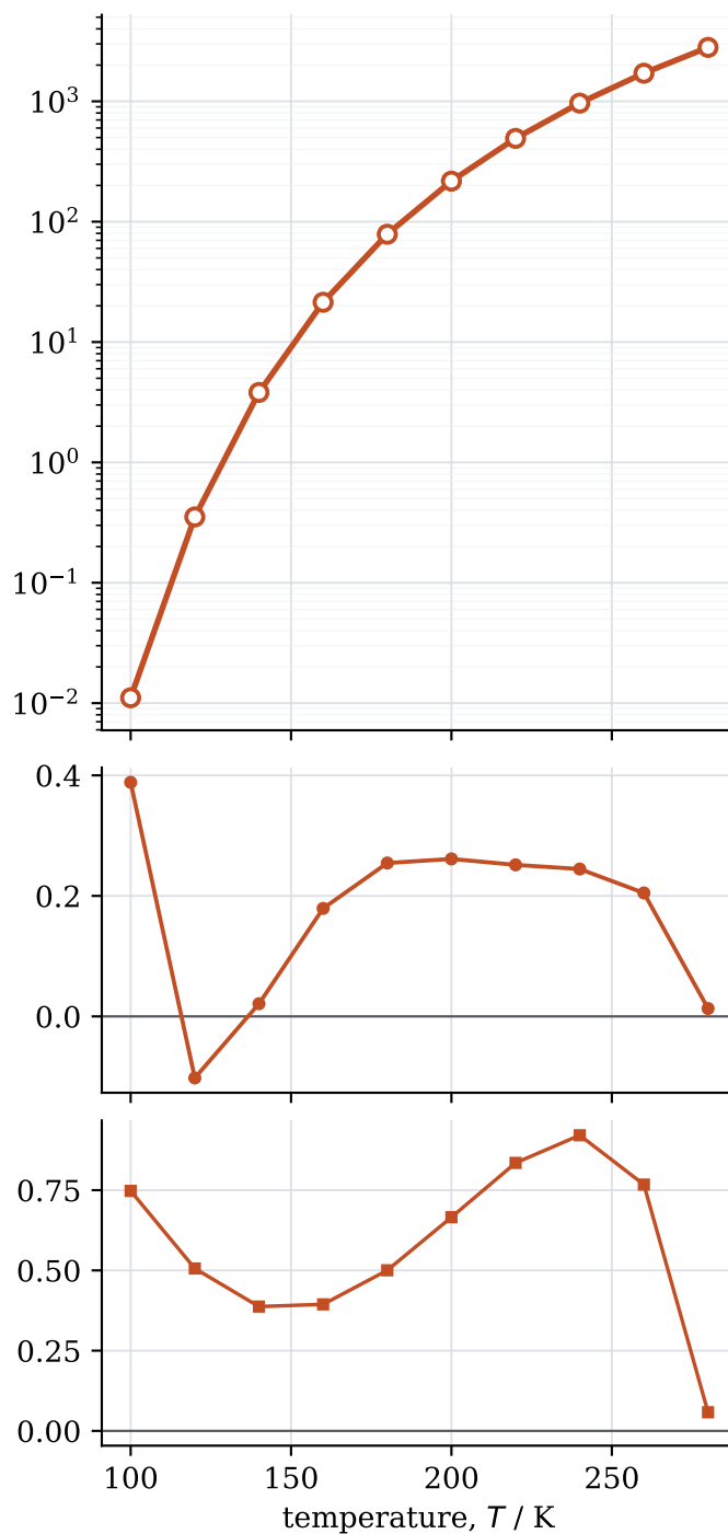
Ethane
