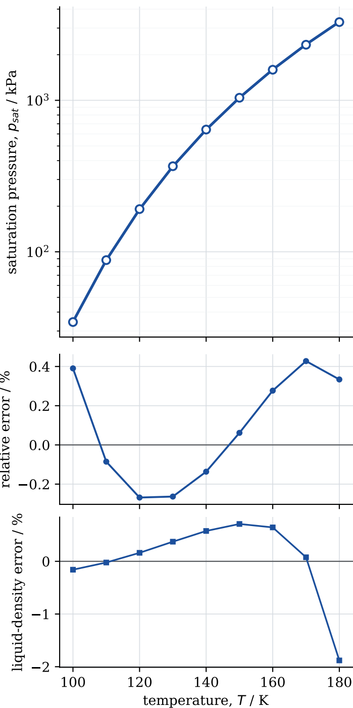
Methane
