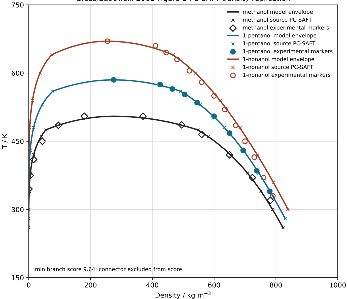
Gross/Sadowski 2002 Figure 1 PC-SAFT density replication
