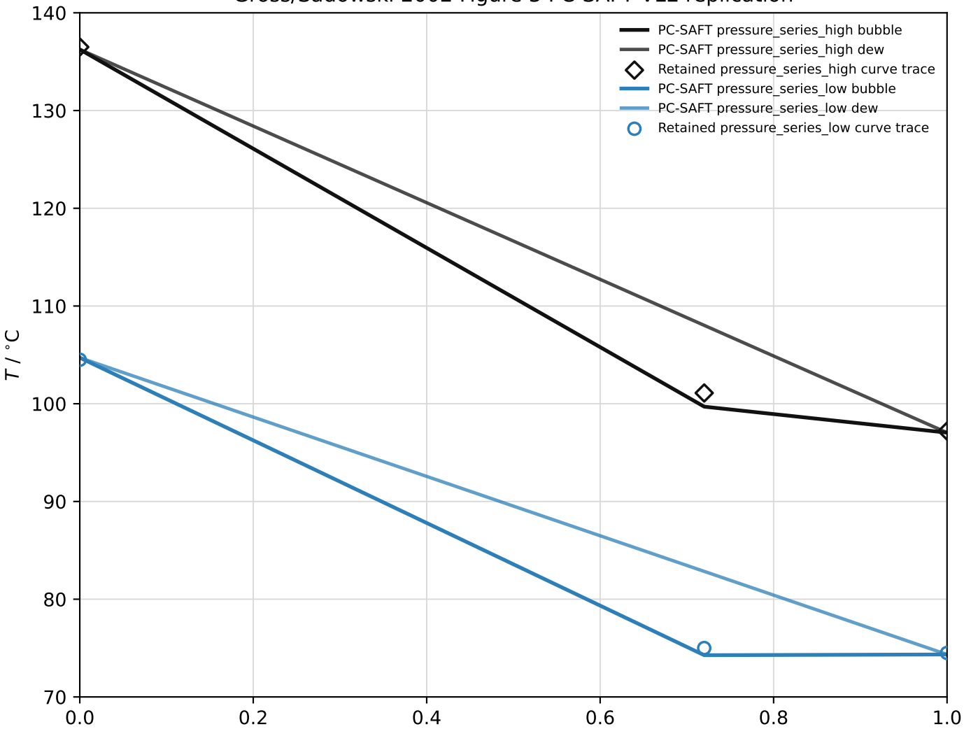
Gross/Sadowski 2002 Figure 3 PC-SAFT VLE replication
