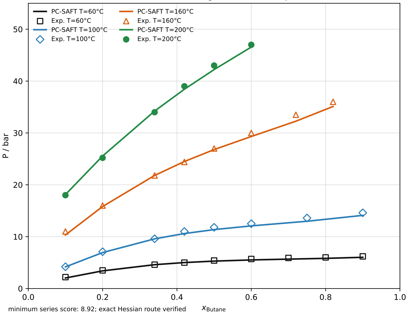
Gross/Sadowski 2002 Figure 6 PC-SAFT replication
