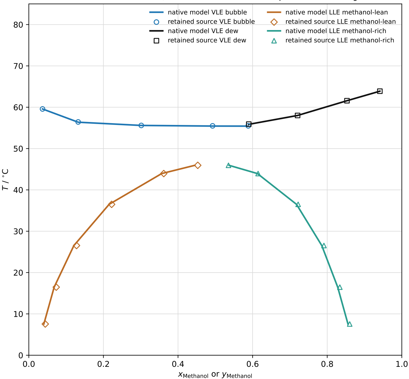
Gross/Sadowski 2002 Figure 8 PC-SAFT replication Minimum branch score: 8.79; lower LLE is an internal sampled-candidate diagnostic
