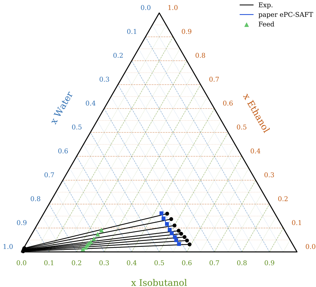
Figure 3. LLE for the system water + ethanol + isobutanol + 5 wt % NaCl at 303.15 K and atmospheric pressure expressed as salt-free composition: black (exp), package internal validation rejected all model tie-lines; no red model tie-lines are drawn, blue squares (paper ePC-SAFT organic branch, 8 points), and green (feed compositions).
