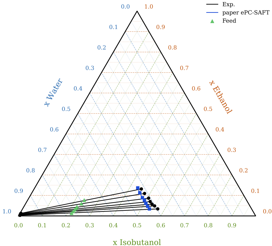
Figure 4. LLE for the system water + ethanol + isobutanol + 5 wt % NaCl at 313.15 K and atmospheric pressure expressed as salt-free composition: black (exp), package internal validation rejected all model tie-lines; no red model tie-lines are drawn, blue squares (paper ePC-SAFT organic branch, 7 points), and green (feed compositions).
