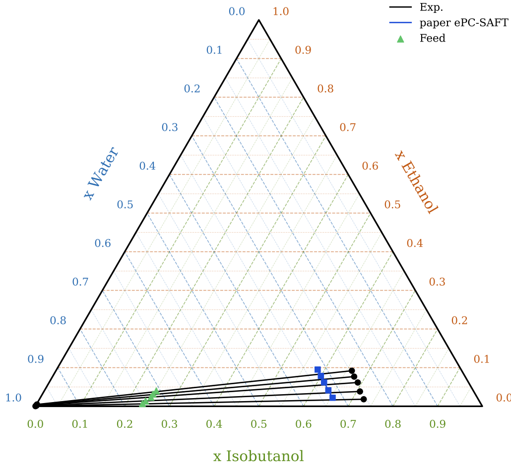
Figure 5. LLE for the system water + ethanol + isobutanol + 10 wt % NaCl at 293.15 K and atmospheric pressure expressed as salt-free composition: black (exp), package internal validation rejected all model tie-lines; no red model tie-lines are drawn, blue squares (paper ePC-SAFT organic branch, 5 points), and green (feed compositions).
